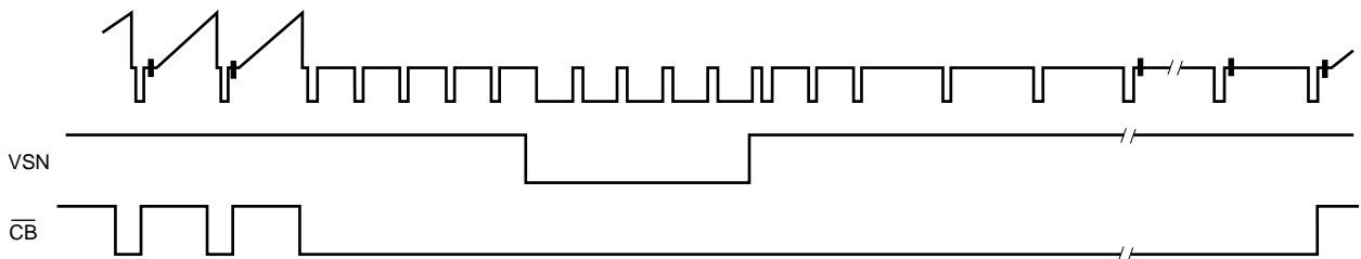
(b) 4th field CVBS output signal
