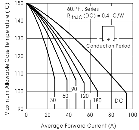
Fig. 2-Current Rating Characteristics
