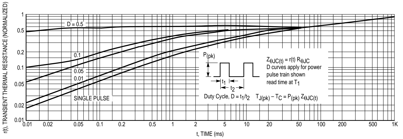
Figure 5. Thermal Response
