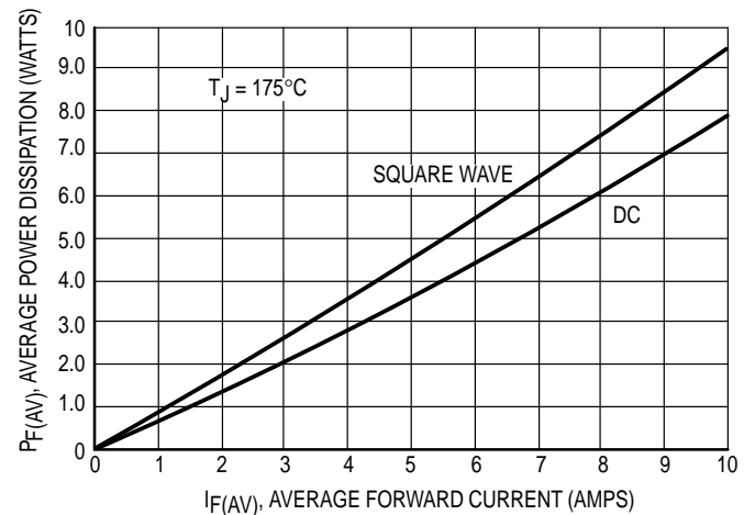
Figure 4. Power Dissipation, Per Leg
