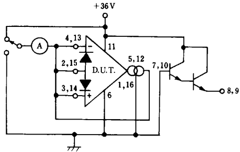
Leakage Current
