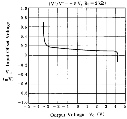
Input Offset Voltage vs. Output Voltage
